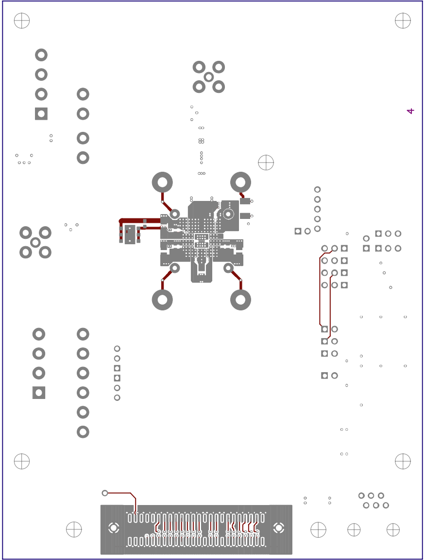
Figure 113. PCB Layout Layer 4, AD973x Evaluation Board, Rev. F
